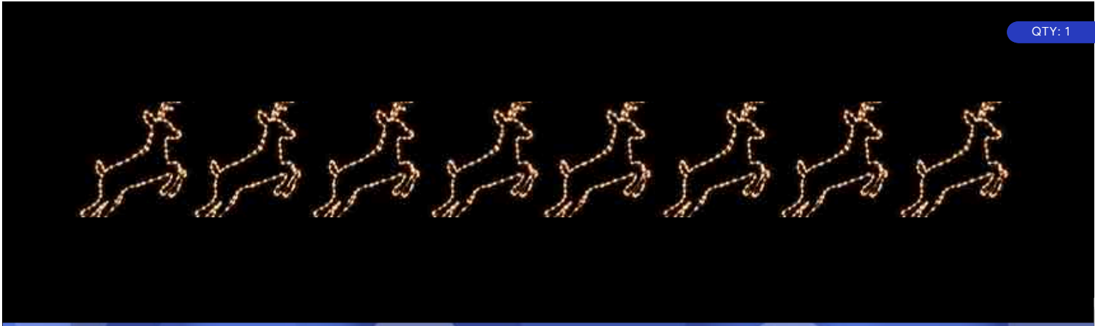
8 REINDEER 15' x 98' | 1496 C7 Lamps LSE-TS-15-8RD
